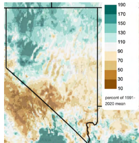
Fig. 4. Percent of average (1991-2020) May precipitation in 2023. ClimateMapper at https://climatetoolbox.org/
