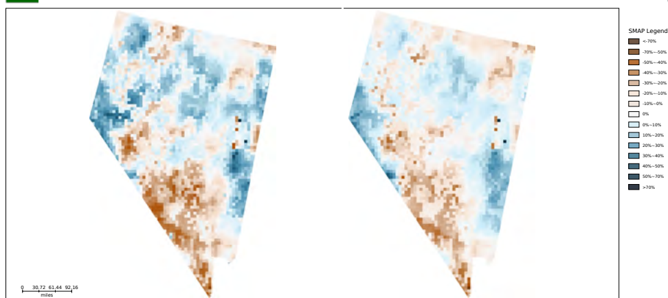
Fig. 7. Topsoil (left) and subsoil (right) moisture anomalies from 9km SMAP for May 22-28, 2023. Maps from Crop-CASMA .
